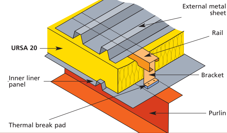
Figure 5 – Roof Detail
