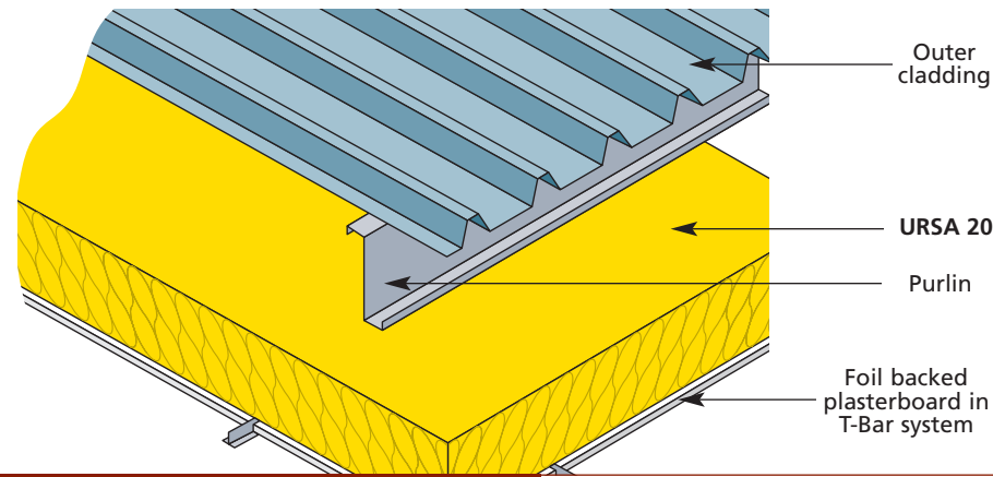
Figure 7 – Suspended Ceilings
