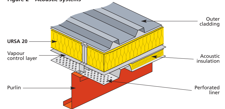
Figure 2 – Acoustic Systems
