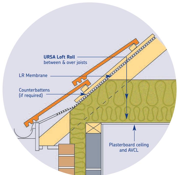
Figure 5 – Non-Ventilated Void
